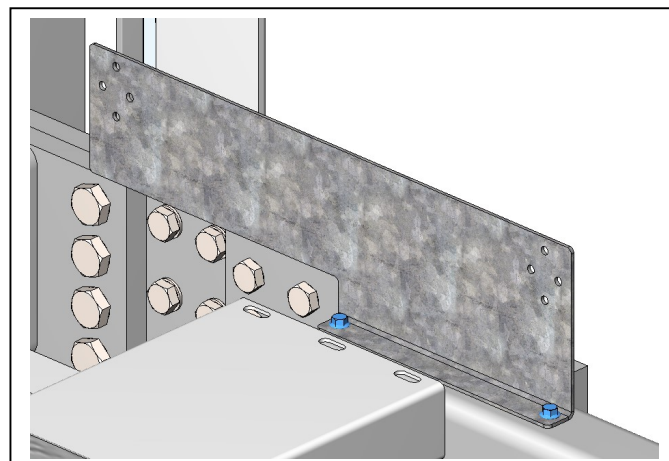
Safety gear Car frame fixation plates
