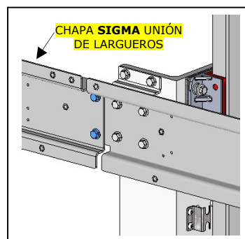
FRONT CAR FRAME PROFILE (DELTA+SIGMA)
