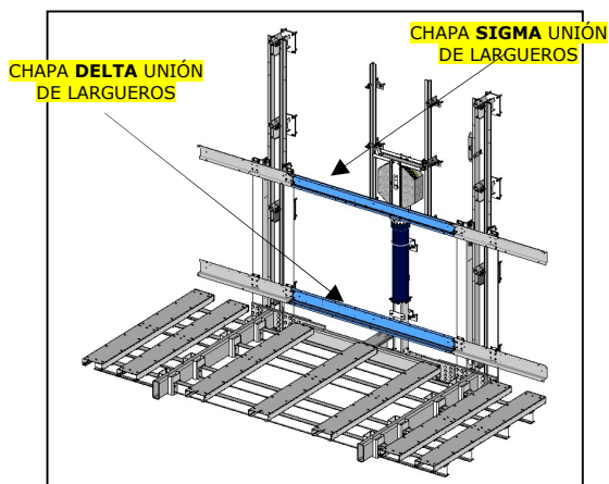
FRONT CAR FRAME PROFILE (DELTA+SIGMA)
